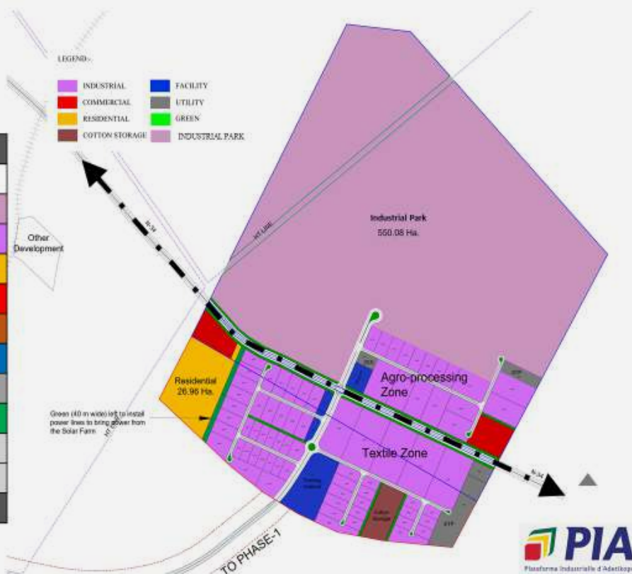
Figure 9: Master plan (Phase 2)
